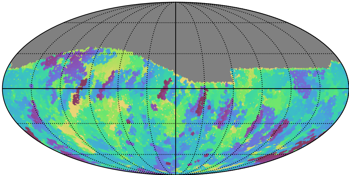
weather_cloudso1v3.4_10yrs Yr 1 r band: Min skyBrightness
