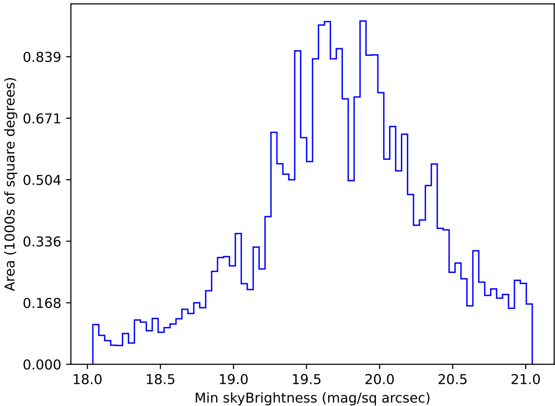
weather_cloudso1v3.4_10yrs Yr 1 r band: Min skyBrightness
