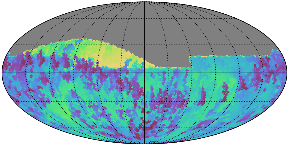
weather_cloudso1v3.4_10yrs Yr 1 all bands: Min skyBrightness
