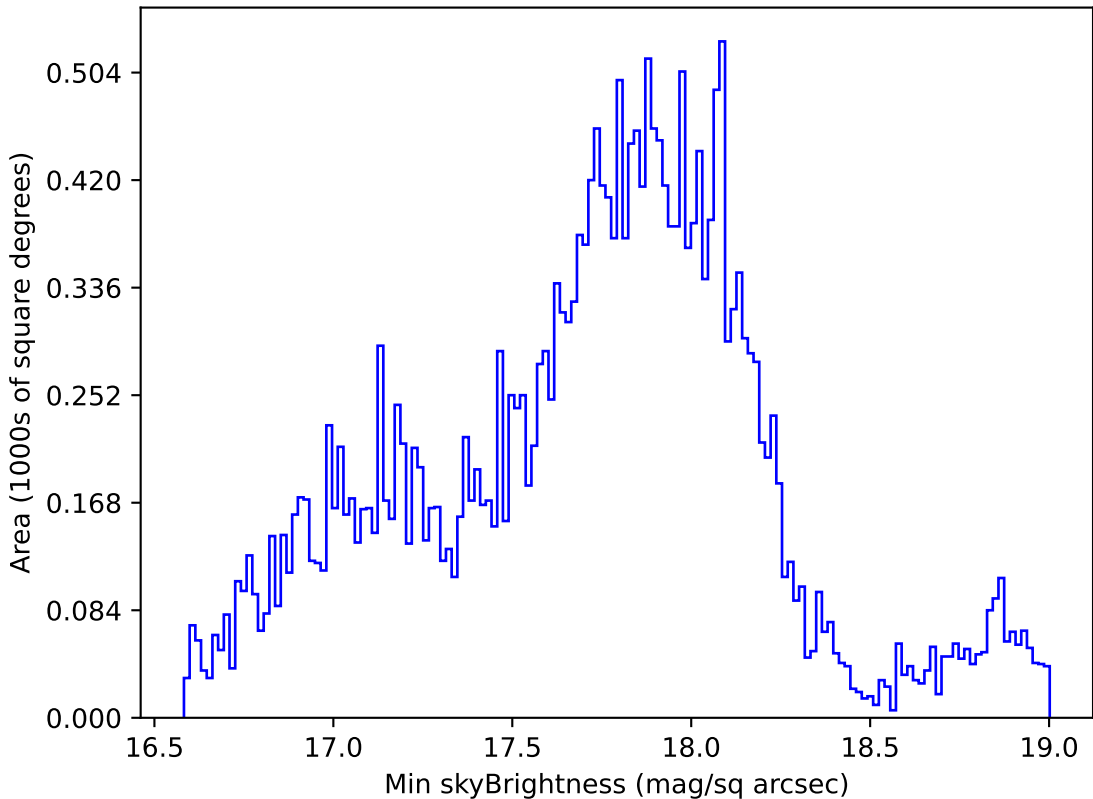
weather_cloudso1v3.4_10yrs Yr 1 all bands: Min skyBrightness
