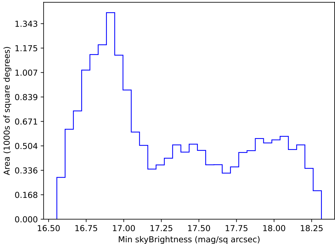
weather_cloudso1v3.4_10yrs WFD z band: Min skyBrightness
