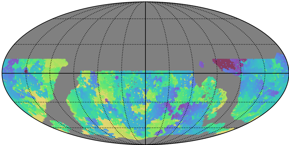
weather_cloudso1v3.4_10yrs WFD u band: Min skyBrightness
