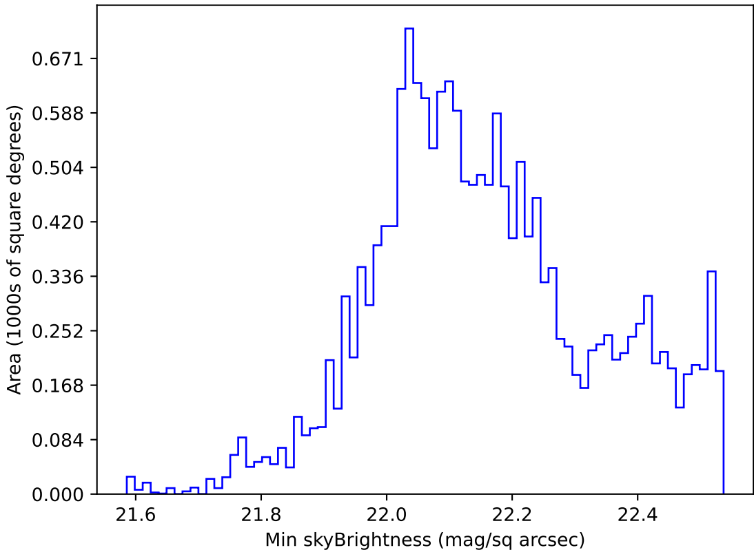
weather_cloudso1v3.4_10yrs WFD u band: Min skyBrightness
