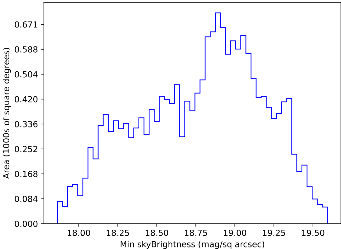
weather_cloudso1v3.4_10yrs WFD r band: Min skyBrightness
