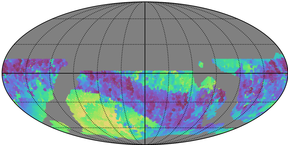
weather_cloudso1v3.4_10yrs WFD i band: Min skyBrightness
