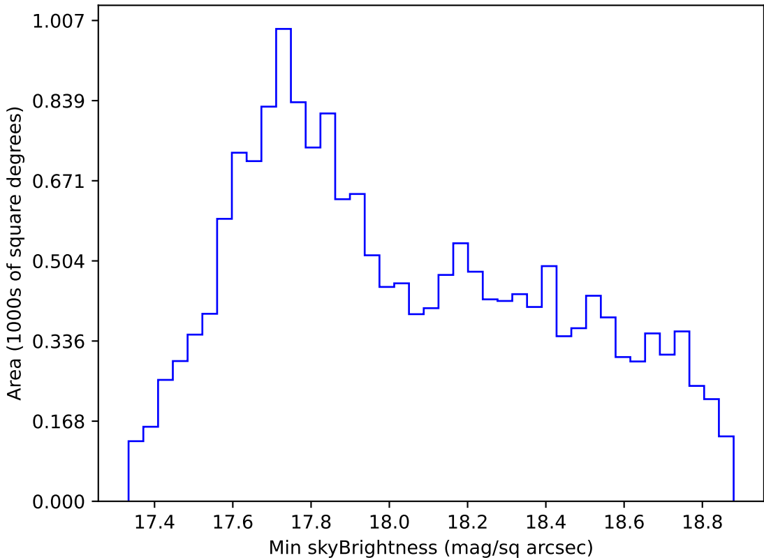
weather_cloudso1v3.4_10yrs WFD i band: Min skyBrightness
