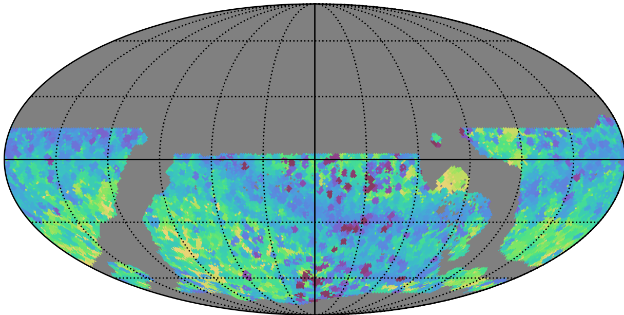
weather_cloudso1v3.4_10yrs WFD all bands: Min skyBrightness
