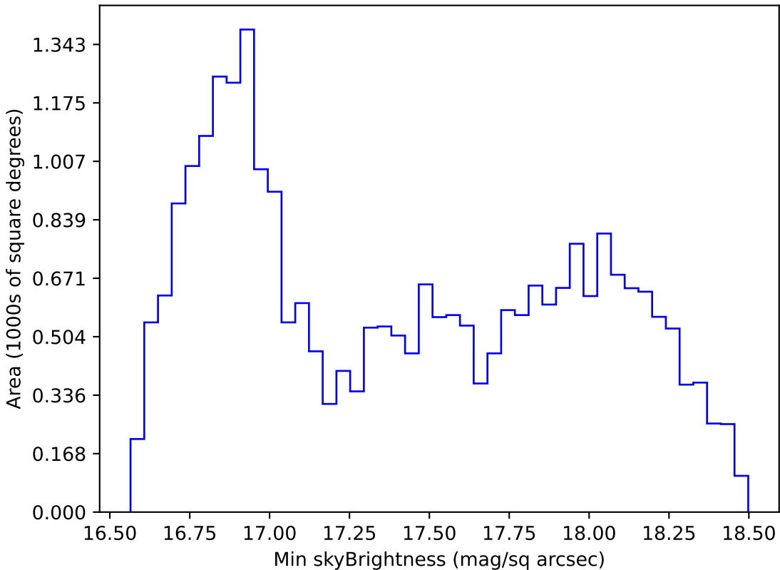
weather_cloudso1v3.4_10yrs All sky z band: Min skyBrightness
