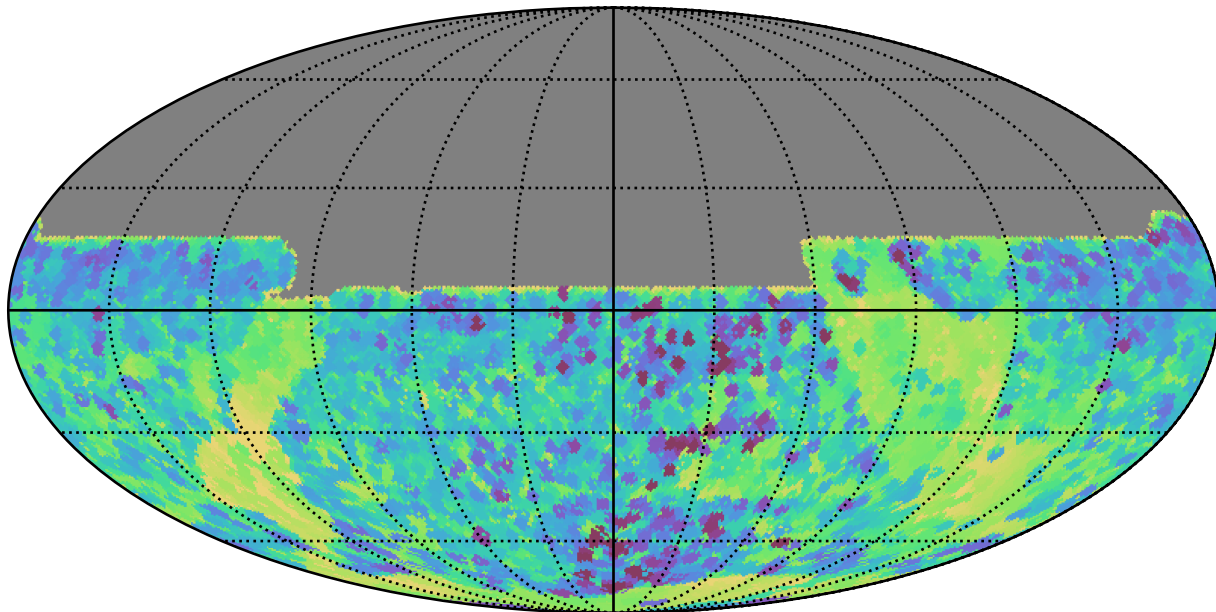
weather_cloudso1v3.4_10yrs All sky y band: Min skyBrightness
