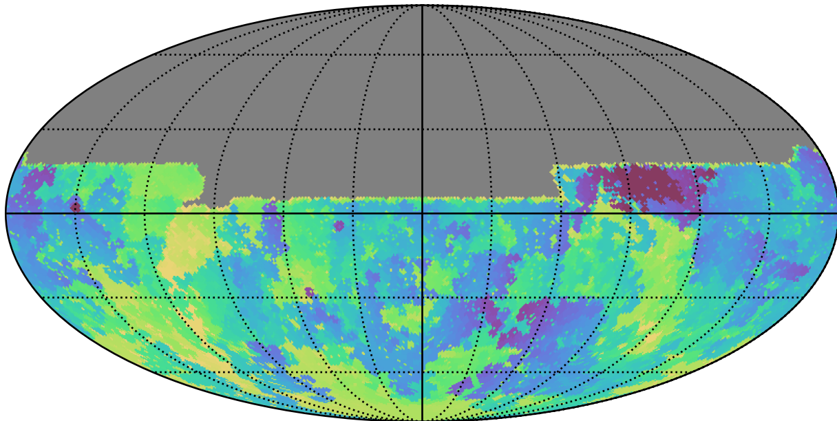
weather_cloudso1v3.4_10yrs All sky u band: Min skyBrightness
