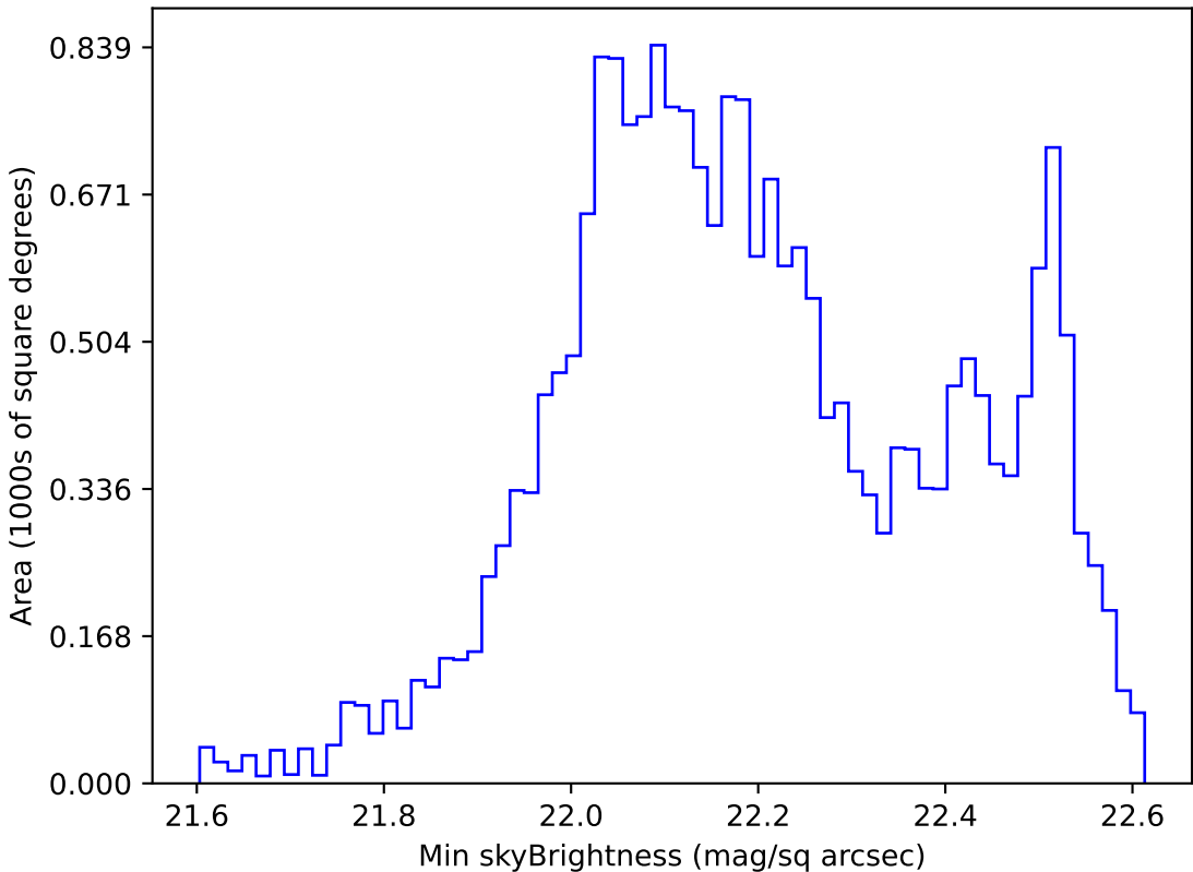
weather_cloudso1v3.4_10yrs All sky u band: Min skyBrightness
