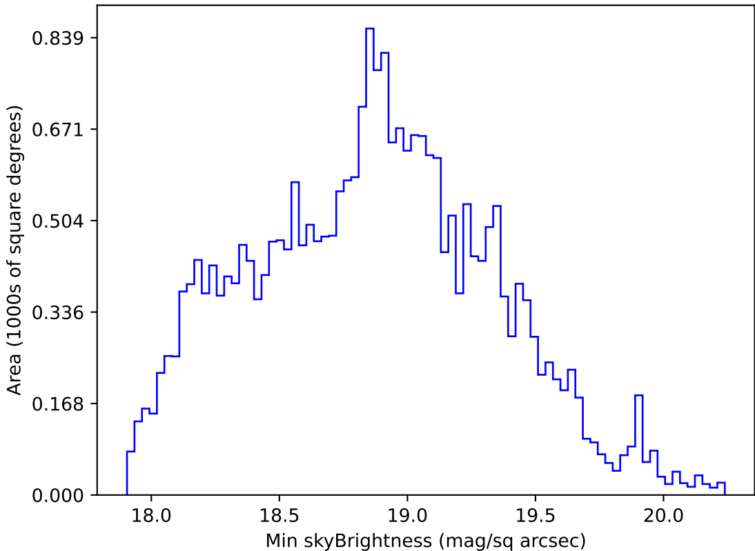
weather_cloudso1v3.4_10yrs All sky r band: Min skyBrightness
