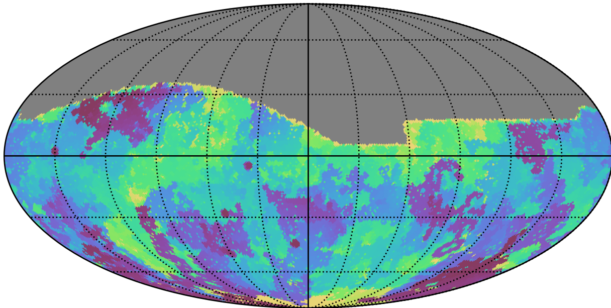
weather_cloudso1v3.4_10yrs All sky g band: Min skyBrightness
