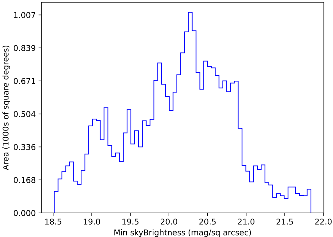
weather_cloudso1v3.4_10yrs All sky g band: Min skyBrightness
