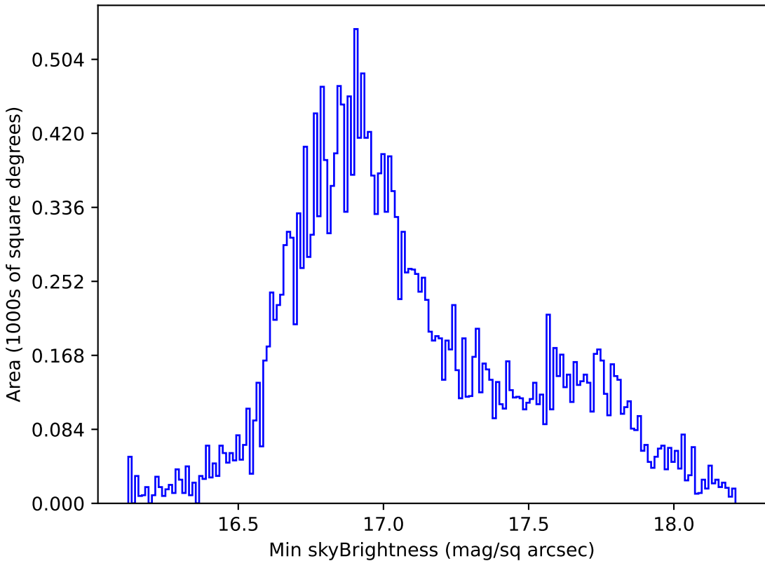
weather_cloudso1v3.4_10yrs All sky all bands: Min skyBrightness
