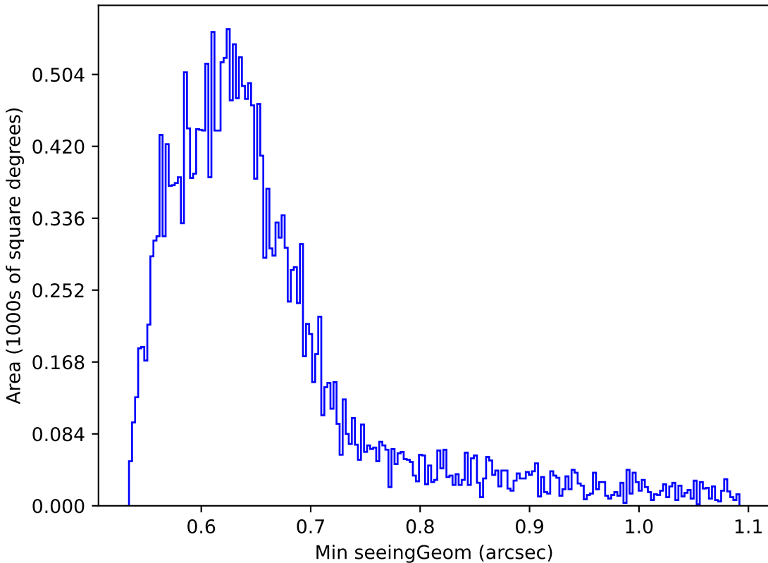
weather_cloudso1v3.4_10yrs Yr 1 z band: Min seeingGeom
