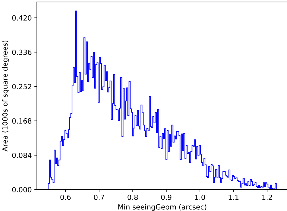
weather_cloudso1v3.4_10yrs Yr 1 u band: Min seeingGeom
