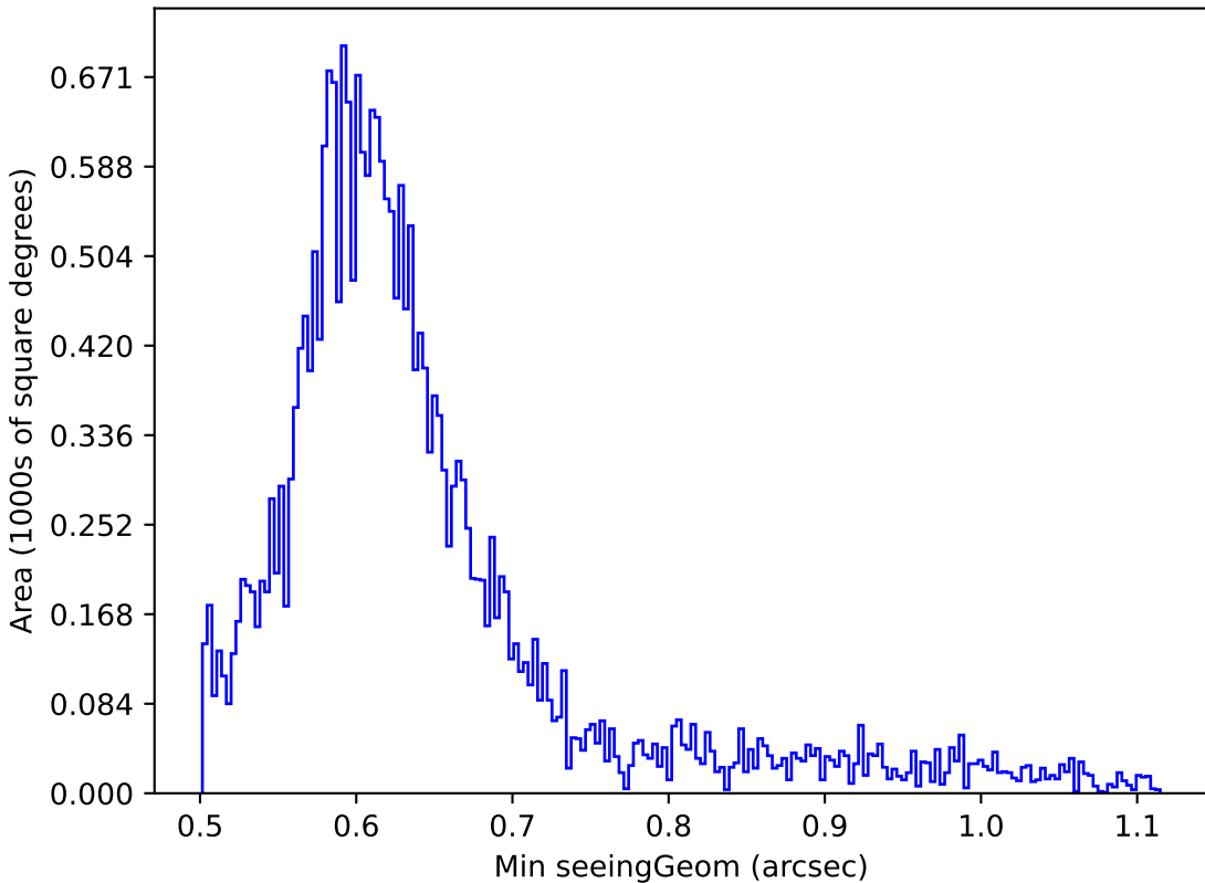
weather_cloudso1v3.4_10yrs Yr 1 r band: Min seeingGeom
