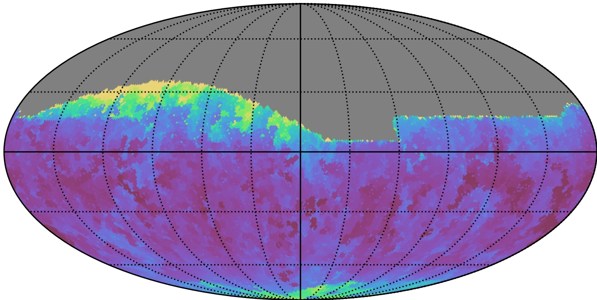
weather_cloudso1v3.4_10yrs Yr 1 all bands: Min seeingGeom
