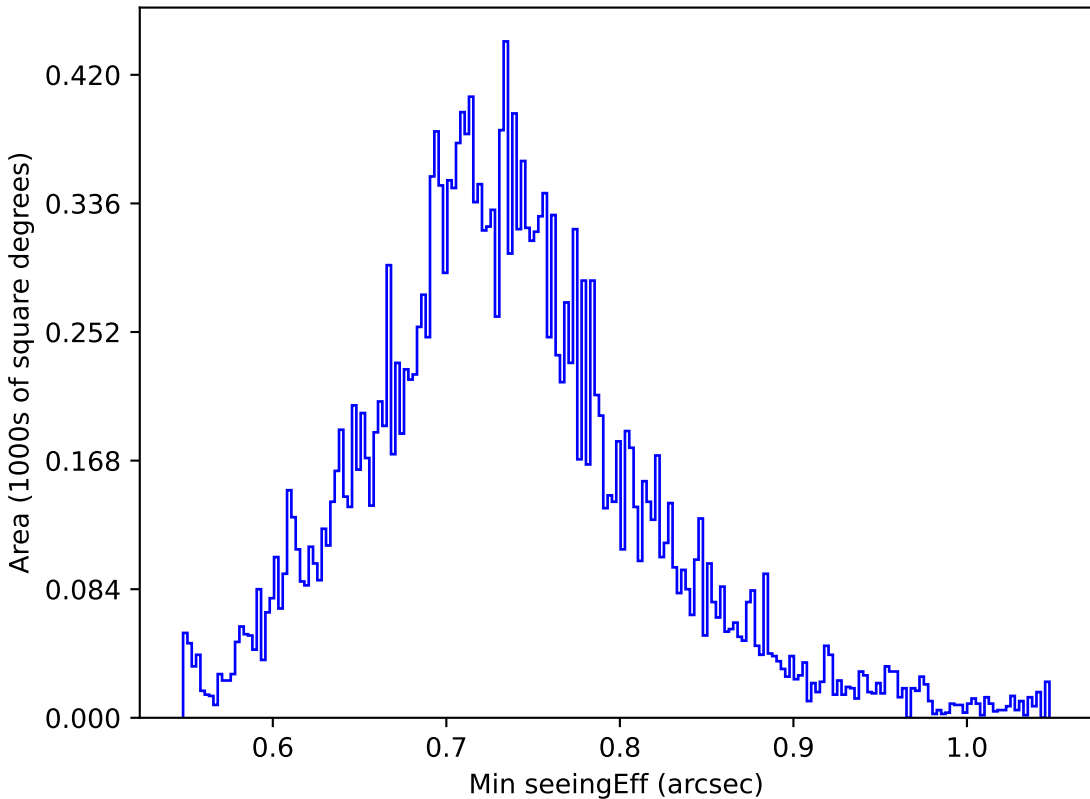
weather_cloudso1v3.4_10yrs Yr 1 y band: Min seeingEff
