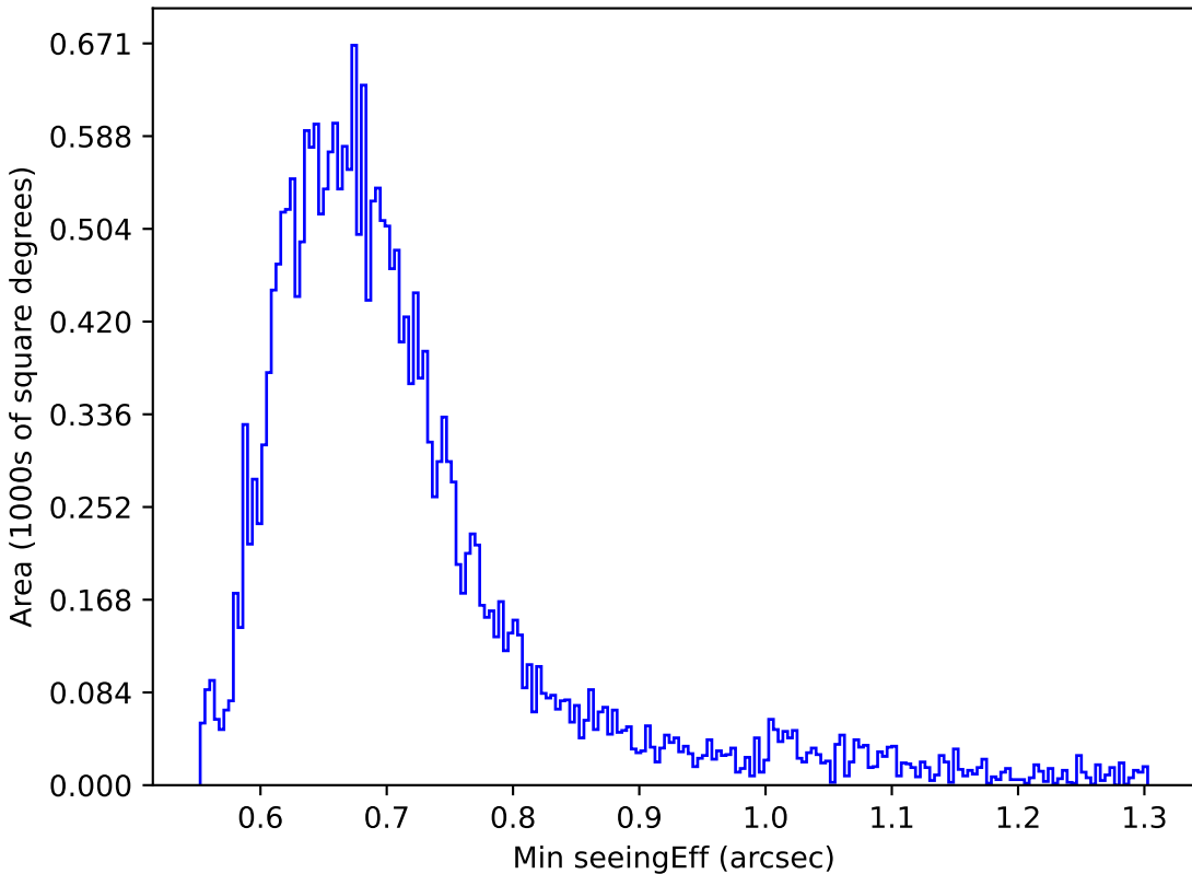
weather_cloudso1v3.4_10yrs Yr 1 i band: Min seeingEff
