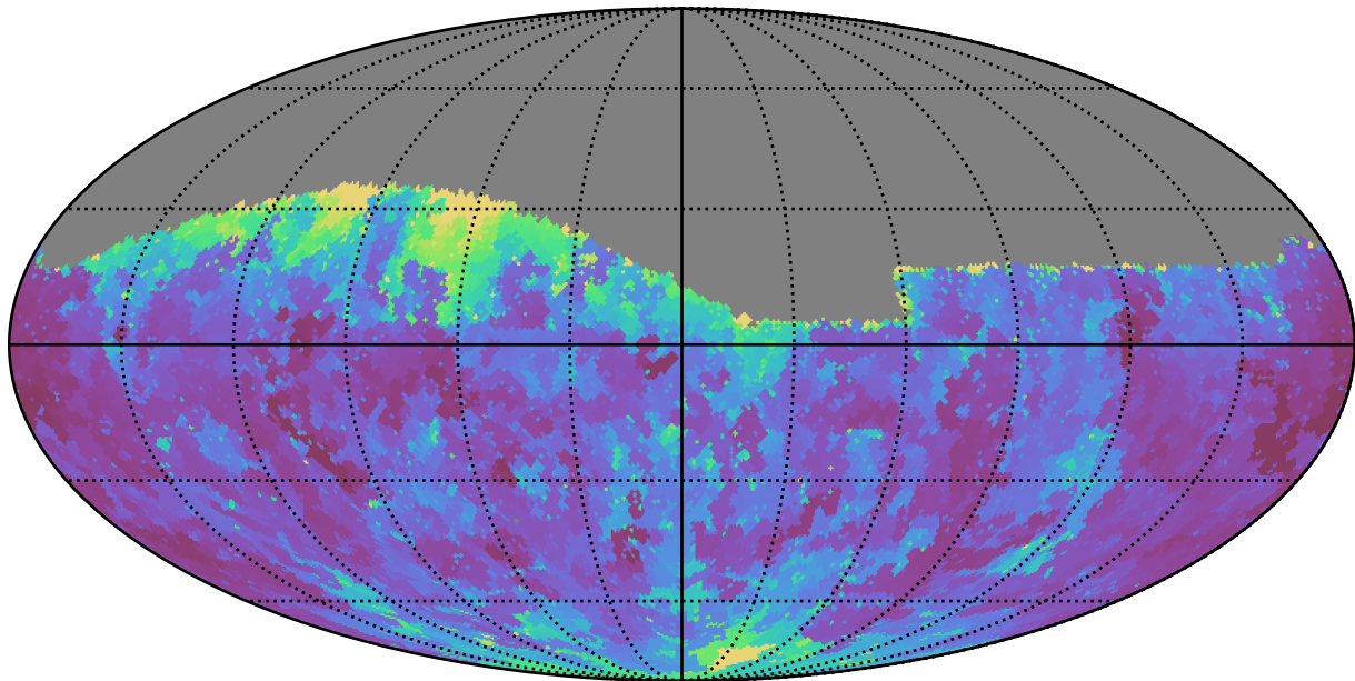
weather_cloudso1v3.4_10yrs Yr 1 g band: Min seeingEff
