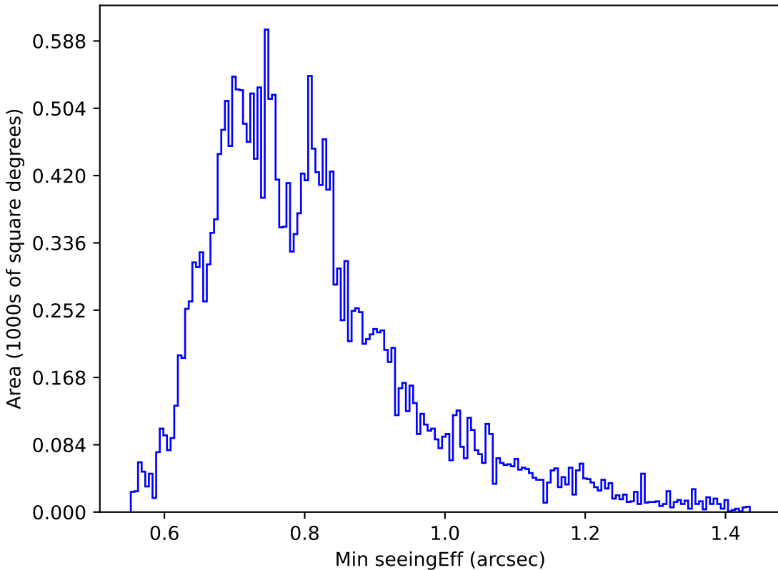
weather_cloudso1v3.4_10yrs Yr 1 g band: Min seeingEff
