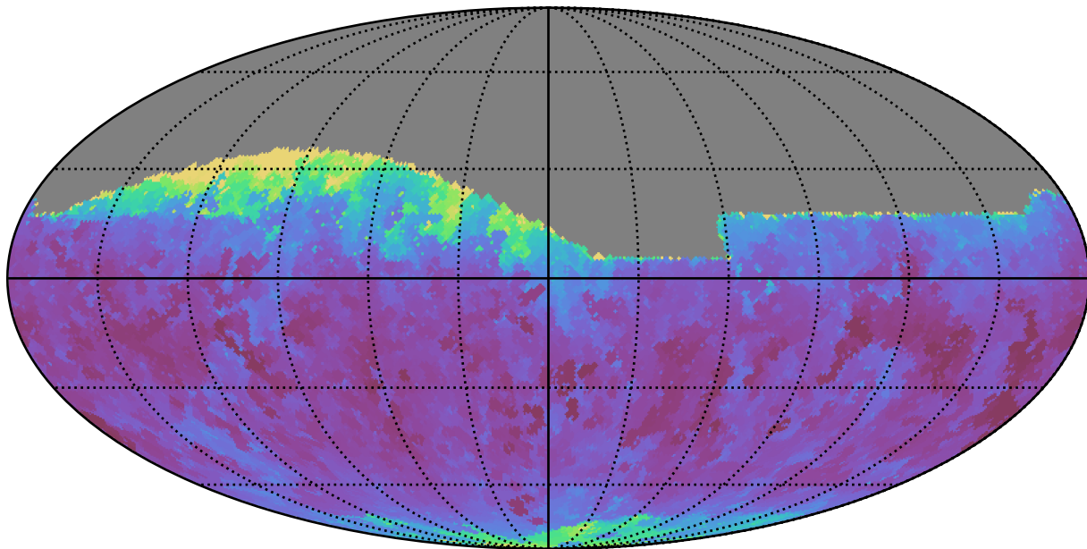
weather_cloudso1v3.4_10yrs Yr 1 all bands: Min seeingEff
