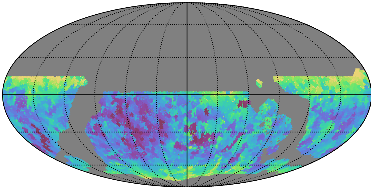
weather_cloudso1v3.4_10yrs WFD z band: Min seeingEff
