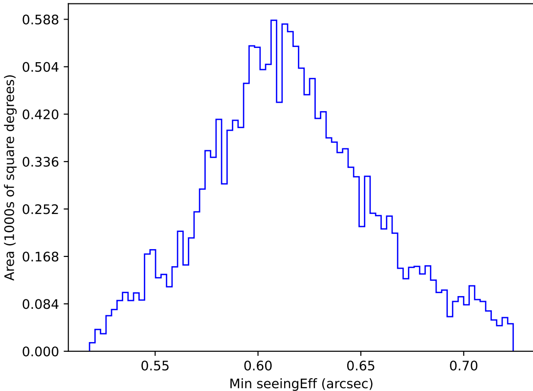
weather_cloudso1v3.4_10yrs WFD z band: Min seeingEff
