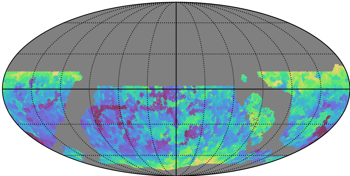
weather_cloudso1v3.4_10yrs WFD y band: Min seeingEff
