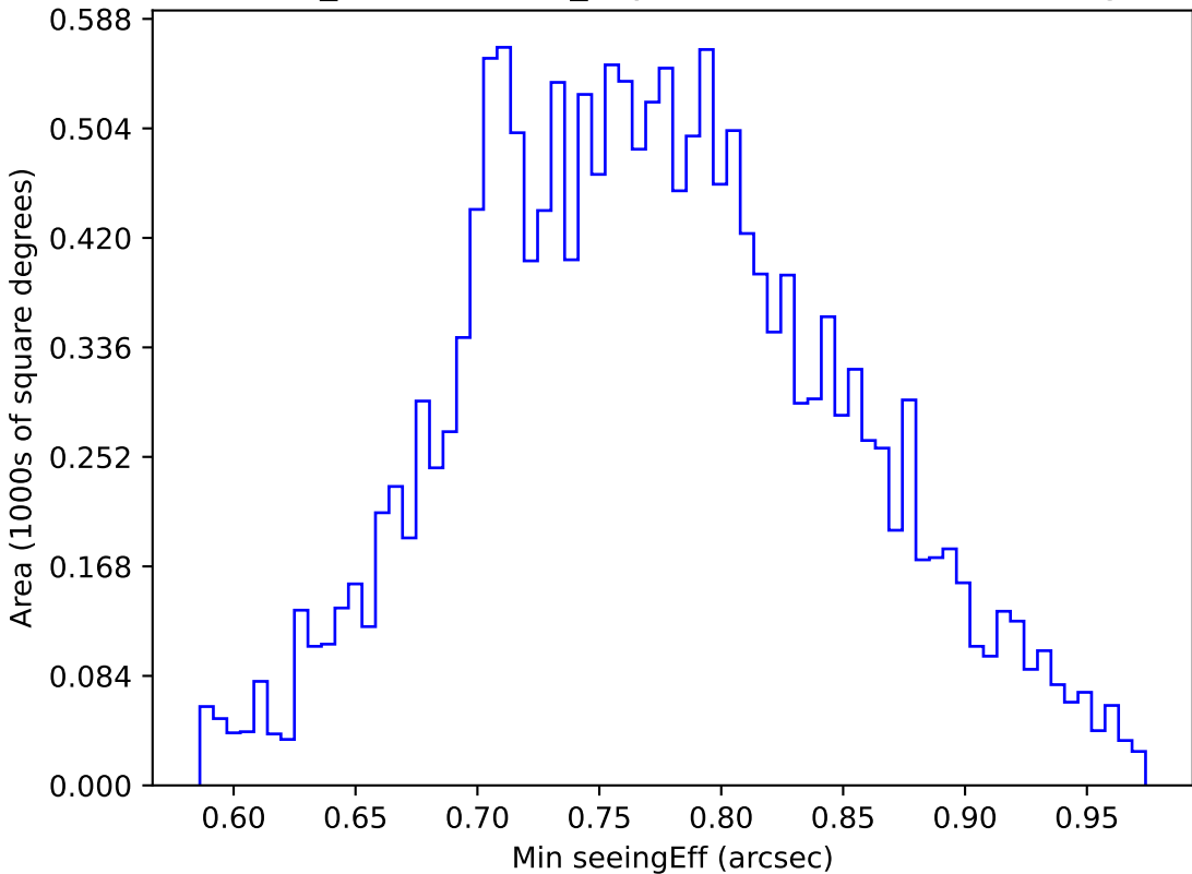
weather_cloudso1v3.4_10yrs WFD u band: Min seeingEff
