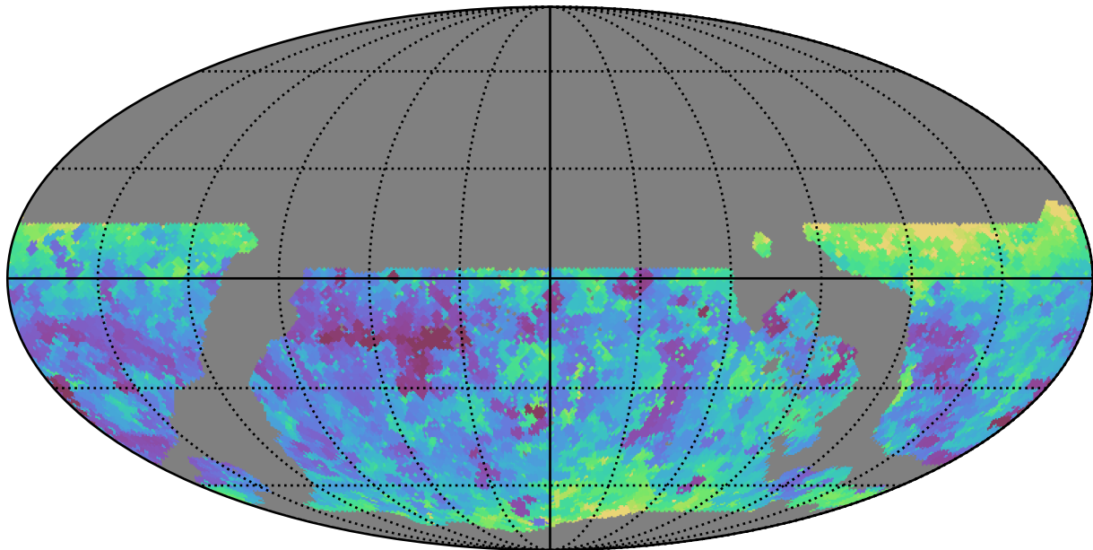
weather_cloudso1v3.4_10yrs WFD r band: Min seeingEff
