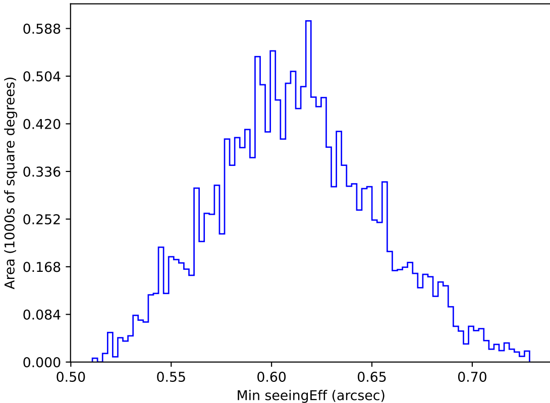
weather_cloudso1v3.4_10yrs WFD r band: Min seeingEff
