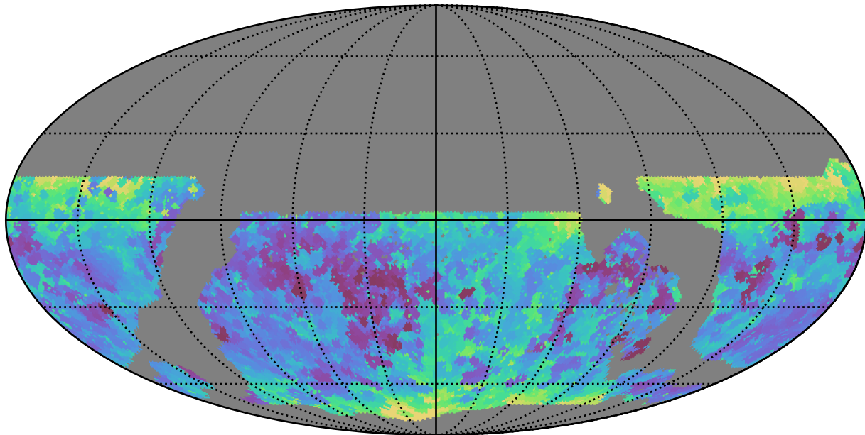
weather_cloudso1v3.4_10yrs WFD i band: Min seeingEff
