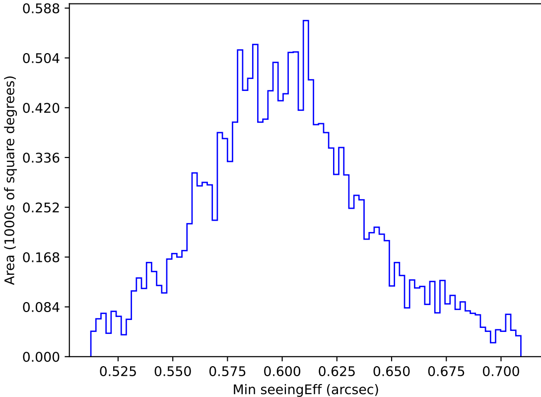
weather_cloudso1v3.4_10yrs WFD i band: Min seeingEff
