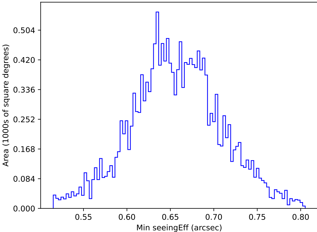
weather_cloudso1v3.4_10yrs WFD g band: Min seeingEff
