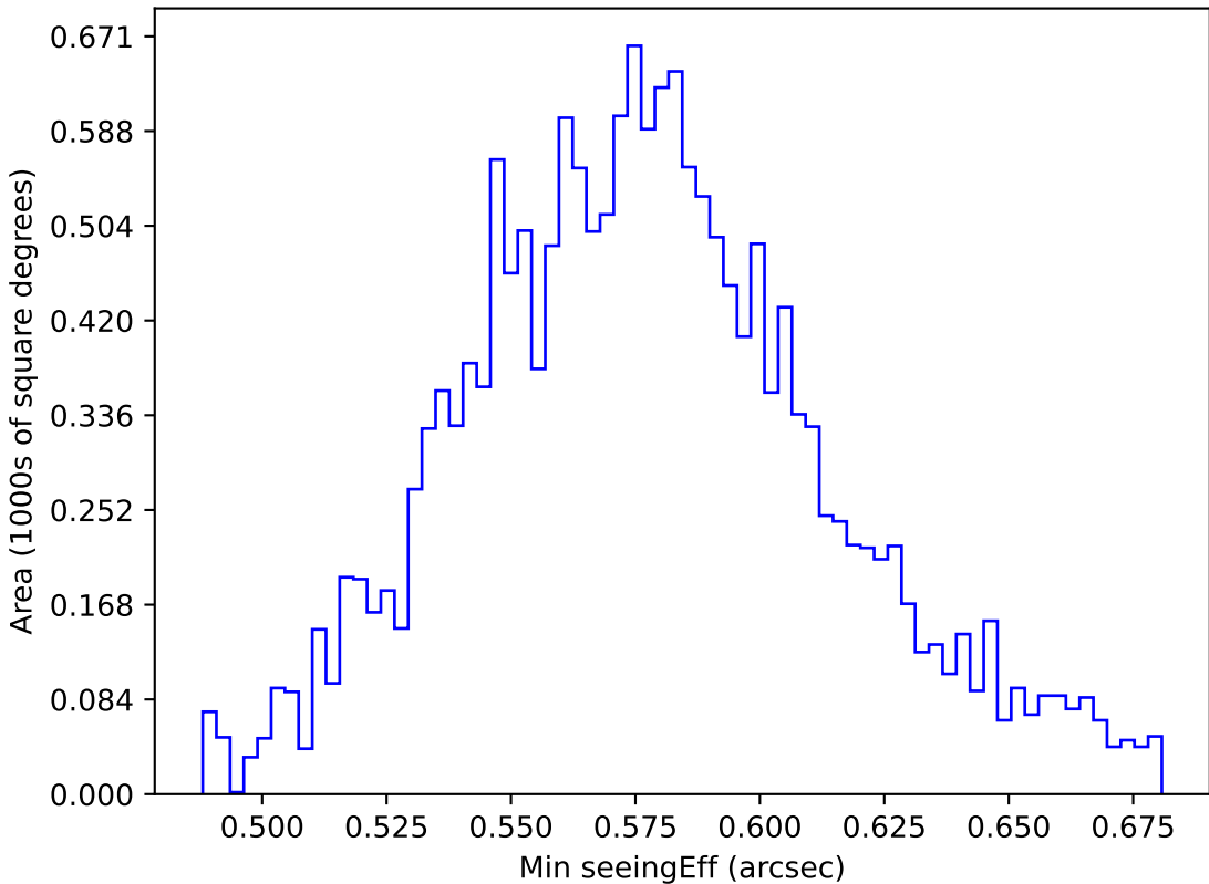
weather_cloudso1v3.4_10yrs WFD all bands: Min seeingEff
