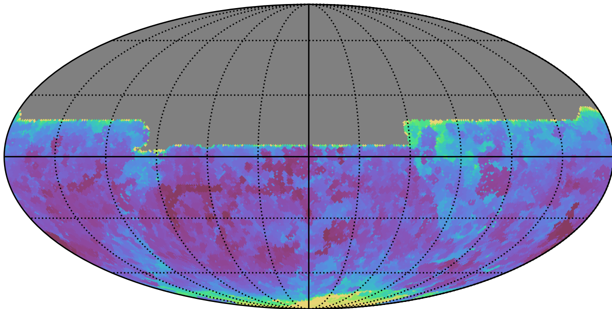
weather_cloudso1v3.4_10yrs All sky y band: Min seeingEff
