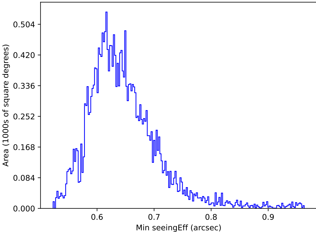
weather_cloudso1v3.4_10yrs All sky y band: Min seeingEff
