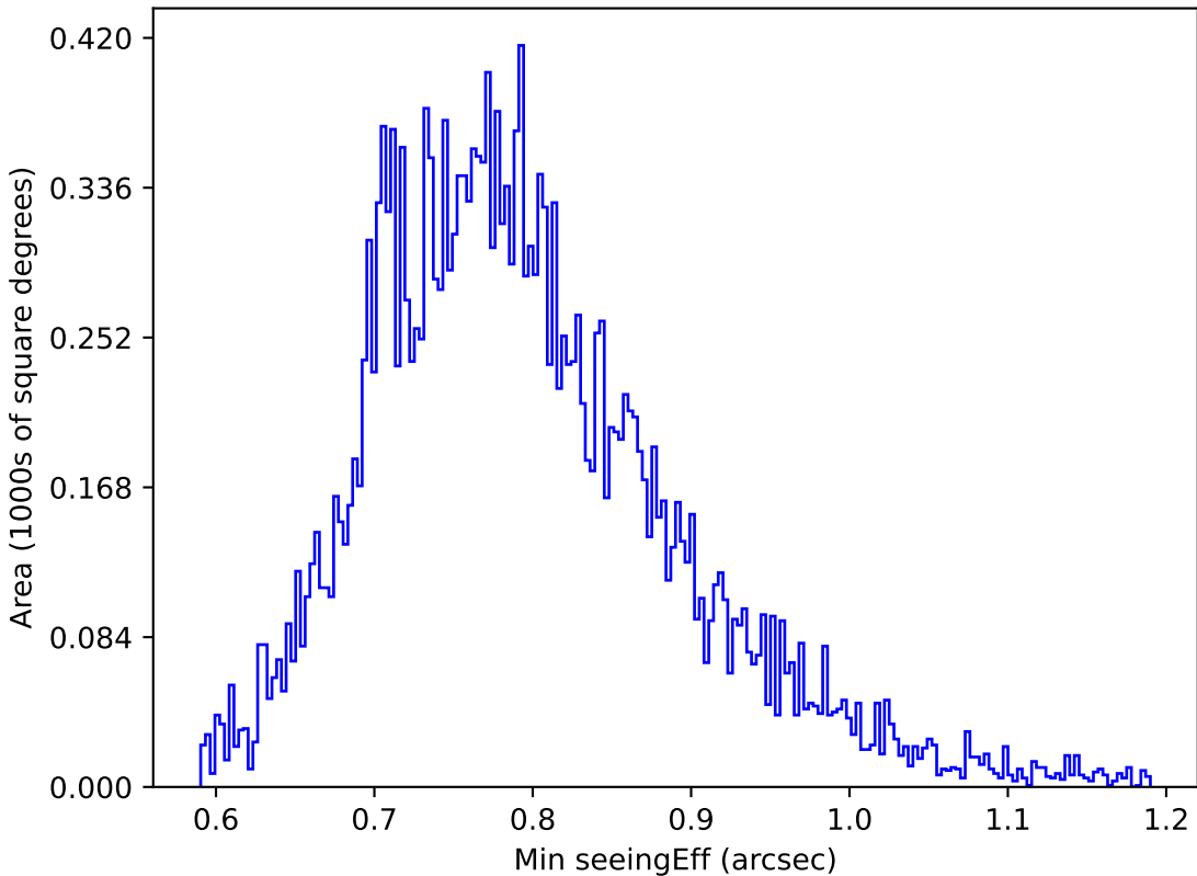
weather_cloudso1v3.4_10yrs All sky u band: Min seeingEff
