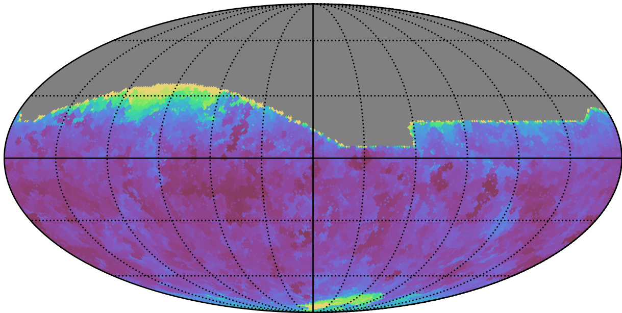
weather_cloudso1v3.4_10yrs All sky r band: Min seeingEff
