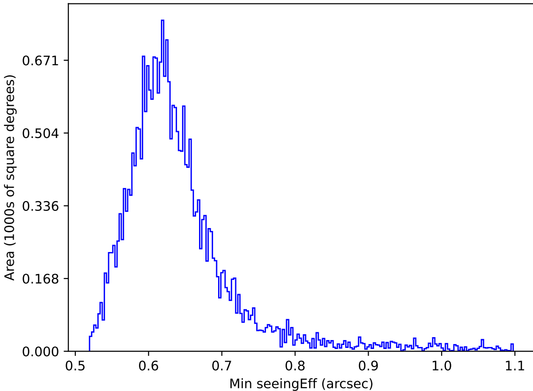
weather_cloudso1v3.4_10yrs All sky r band: Min seeingEff
