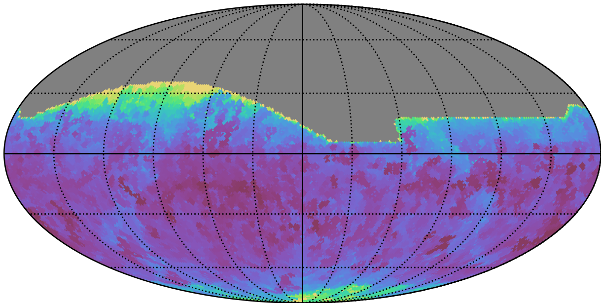
weather_cloudso1v3.4_10yrs All sky all bands: Min seeingEff
