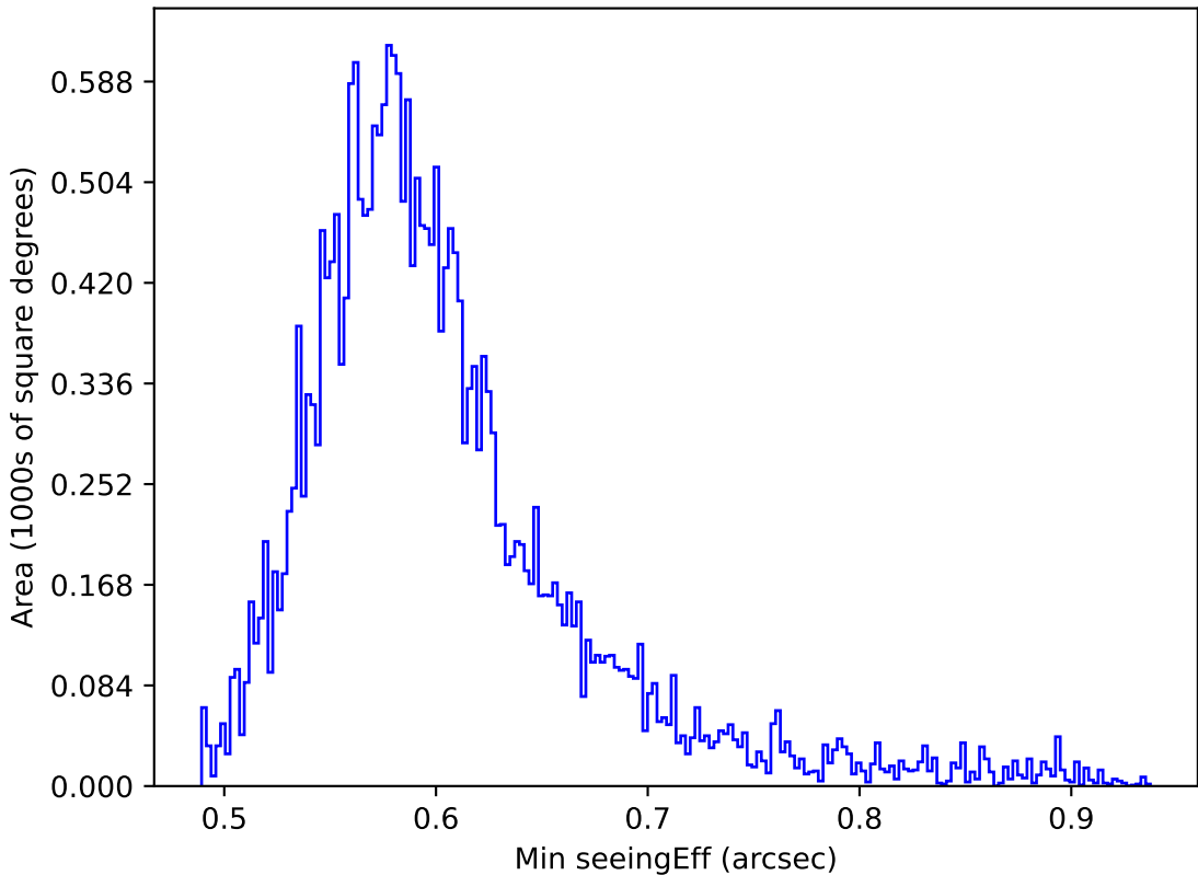
weather_cloudso1v3.4_10yrs All sky all bands: Min seeingEff
