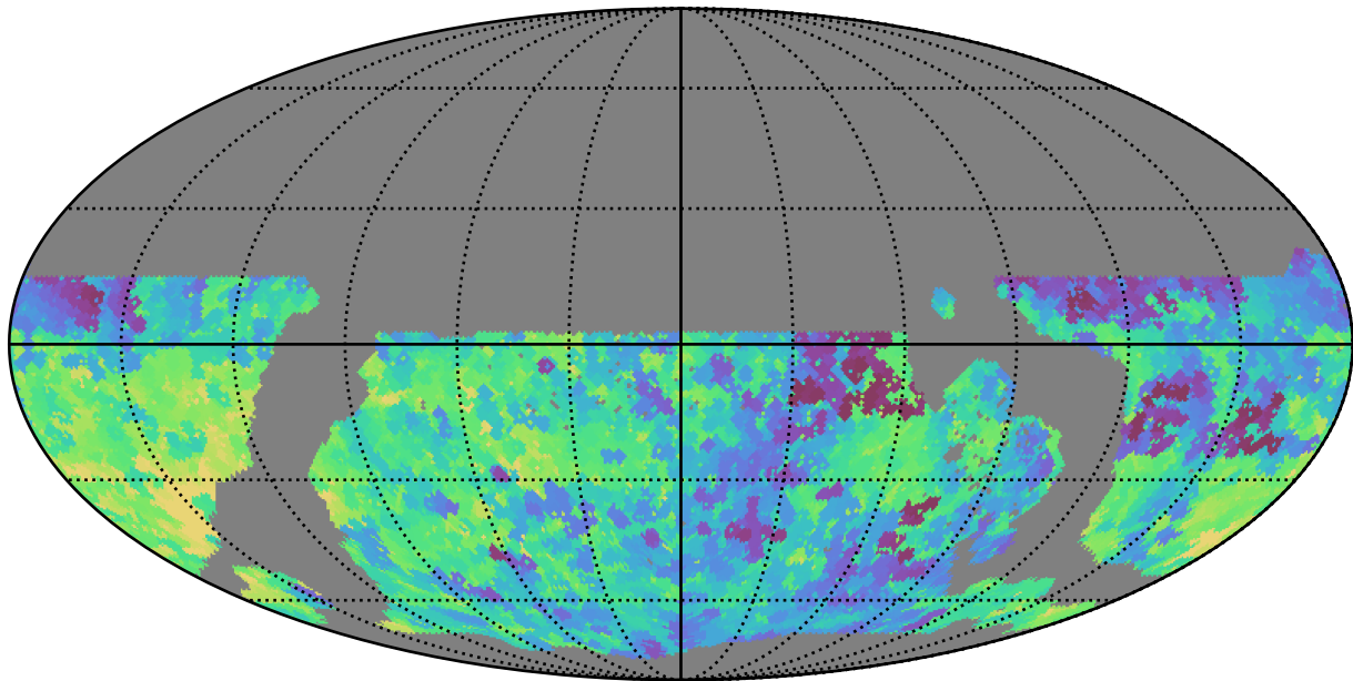
weather_cloudso1v3.4_10yrs WFD all bands: Min saturation_mag
