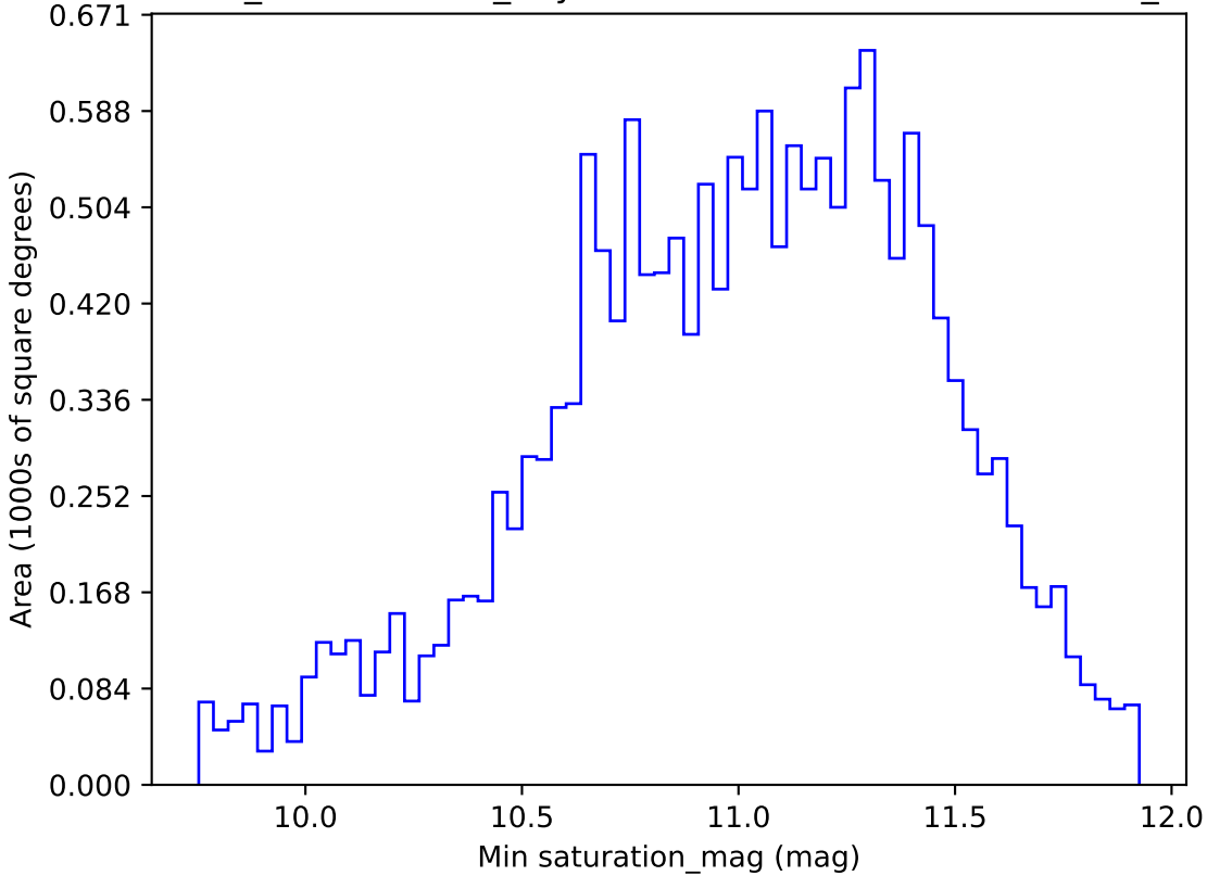
weather_cloudso1v3.4_10yrs WFD all bands: Min saturation_mag
