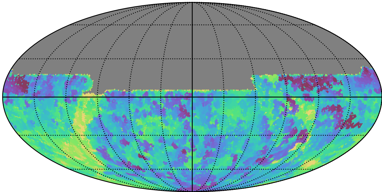
weather_cloudso1v3.4_10yrs All sky u band: Min saturation_mag
