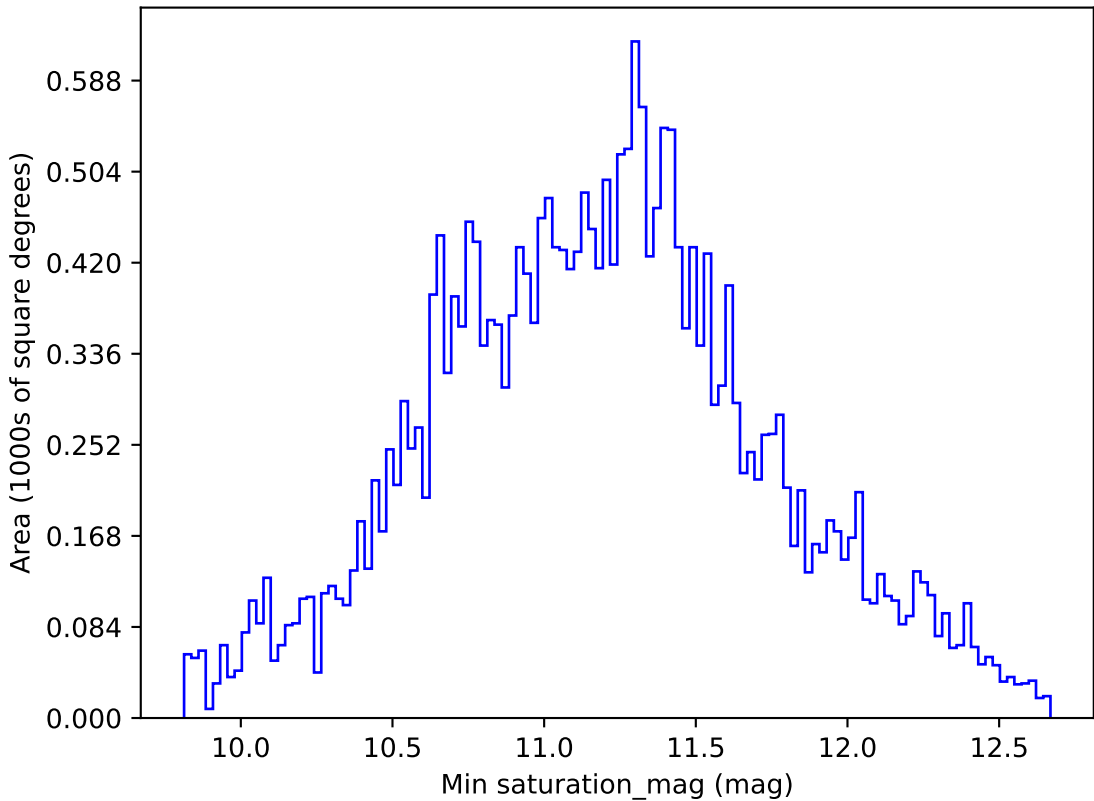
weather_cloudso1v3.4_10yrs All sky all bands: Min saturation_mag
