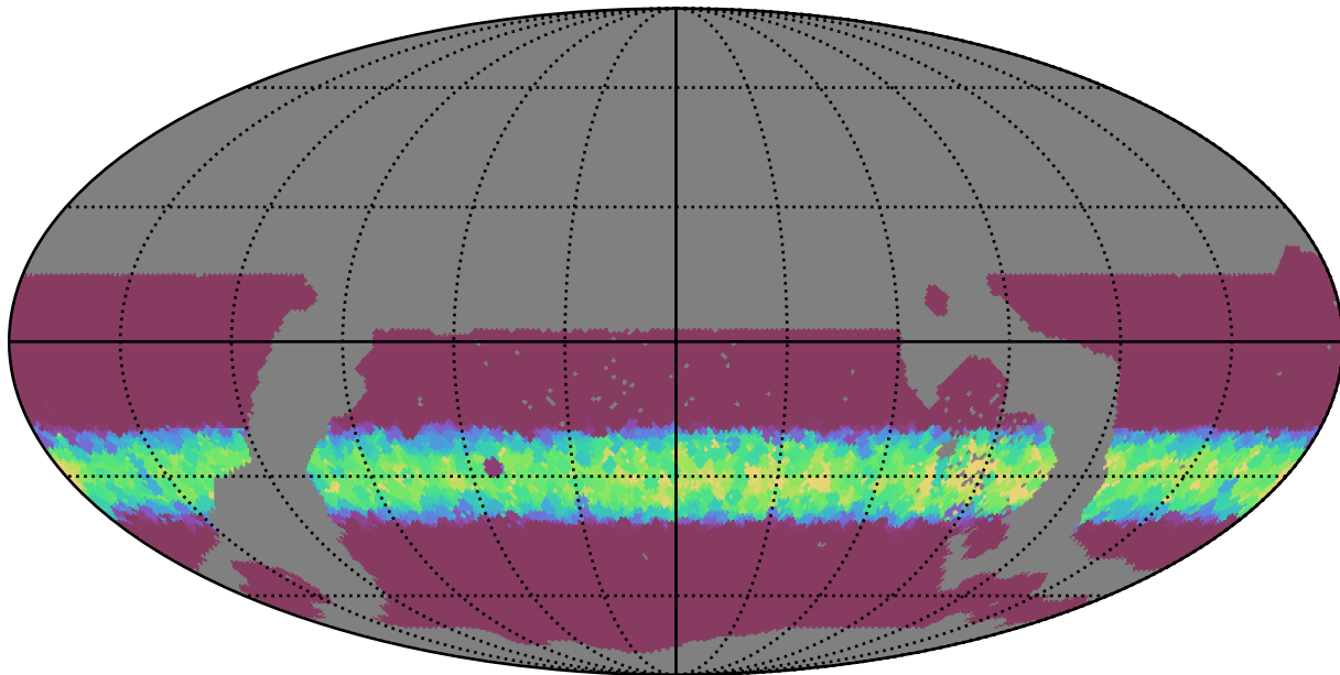
weather_cloudso1v3.4_10yrs WFD z band: Min normairmass
